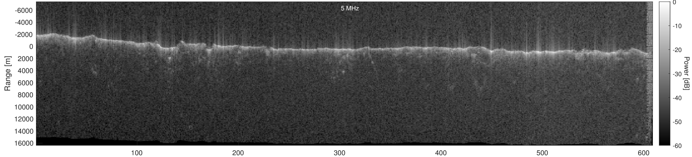
Orbit 18814, Optimized, No Window, Depth-Corrected, Channel 2
