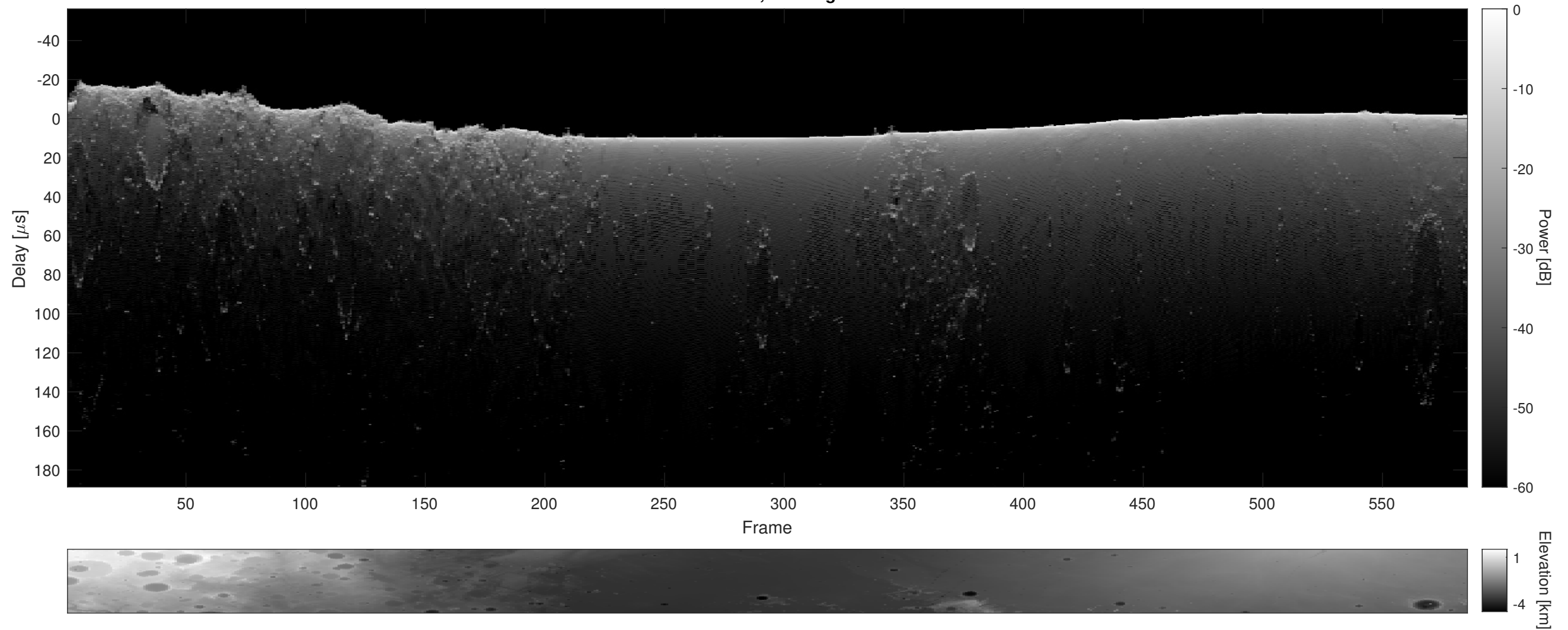
Orbit 18816, Cluttergram
