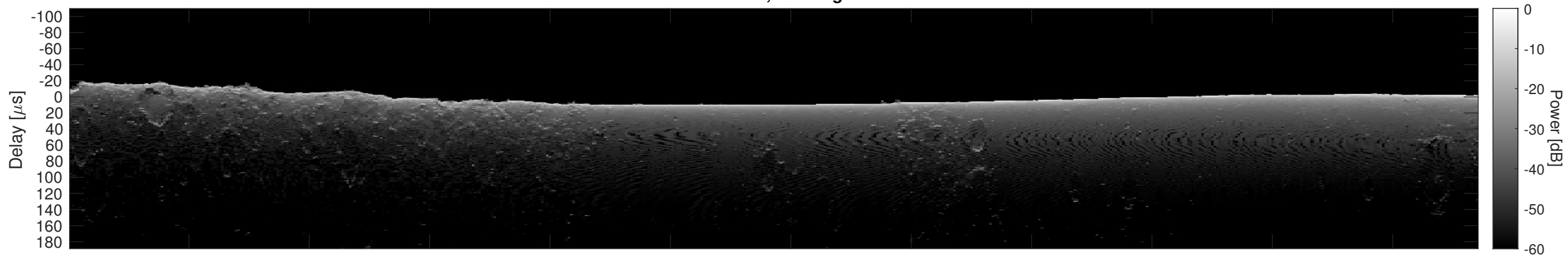
Orbit 18816, Cluttergram
