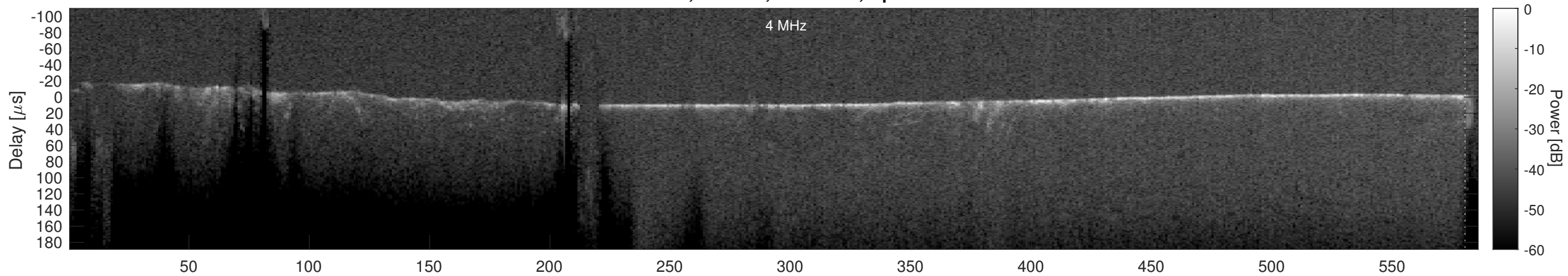
Orbit 18816, Cluttergram
