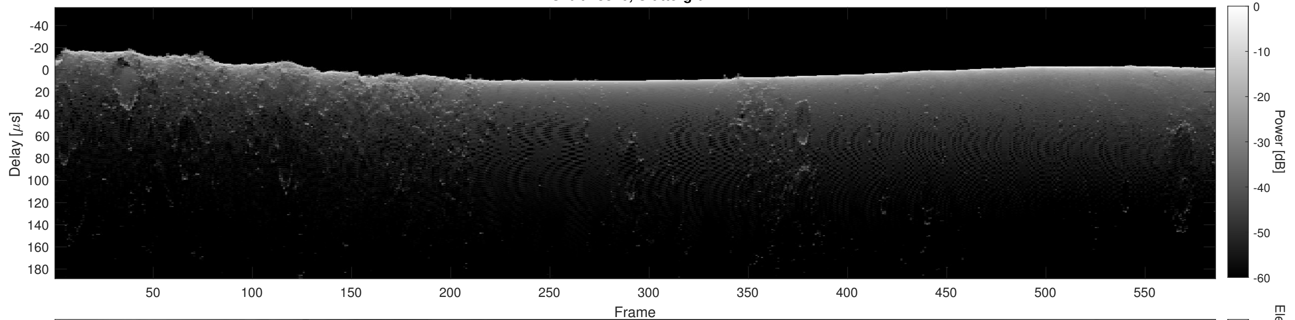
Orbit 18816, Cluttergram
