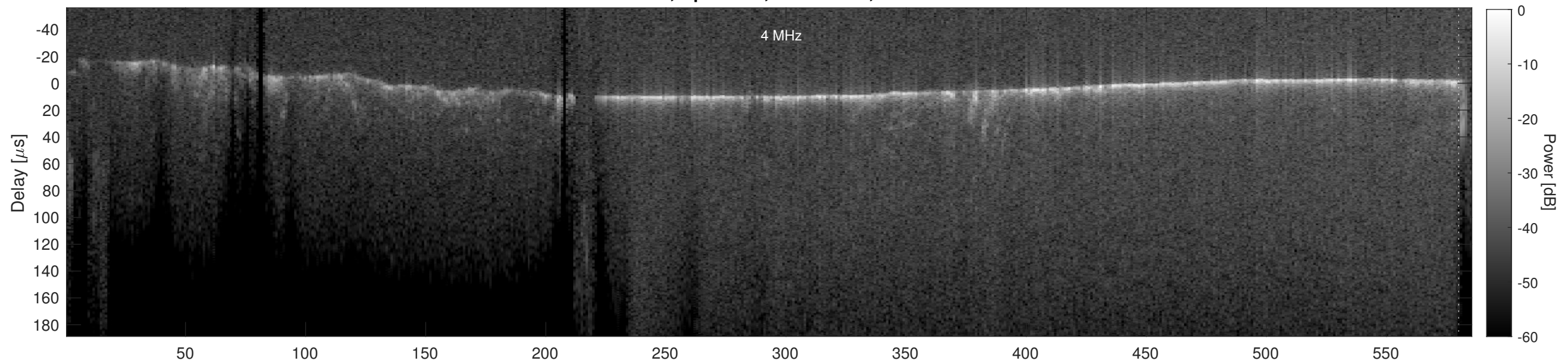
Orbit 18816, Cluttergram
