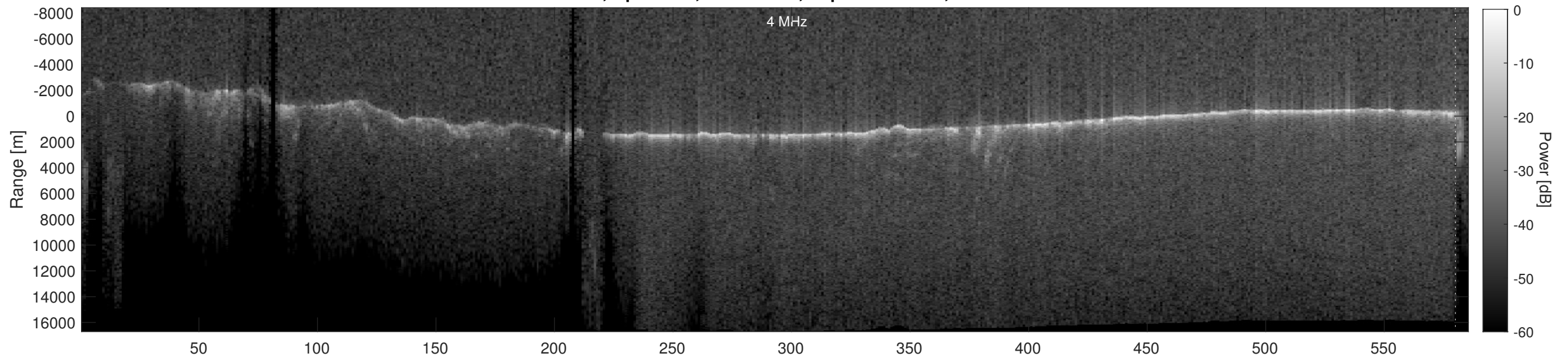
Orbit 18816, Depth-Corrected Cluttergram
