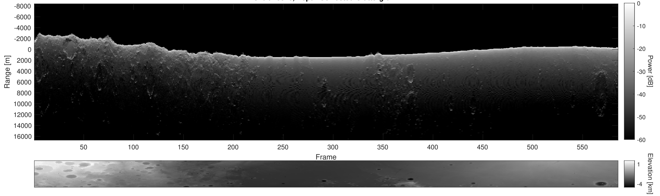
Orbit 18816, Depth-Corrected Cluttergram
