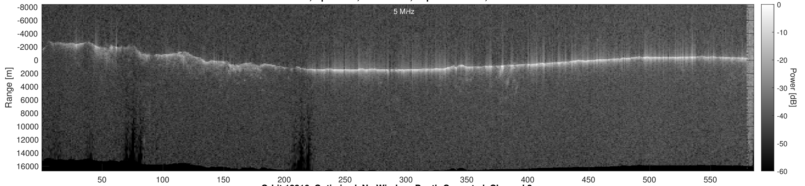
Orbit 18816, Optimized, No Window, Depth-Corrected, Channel 2
