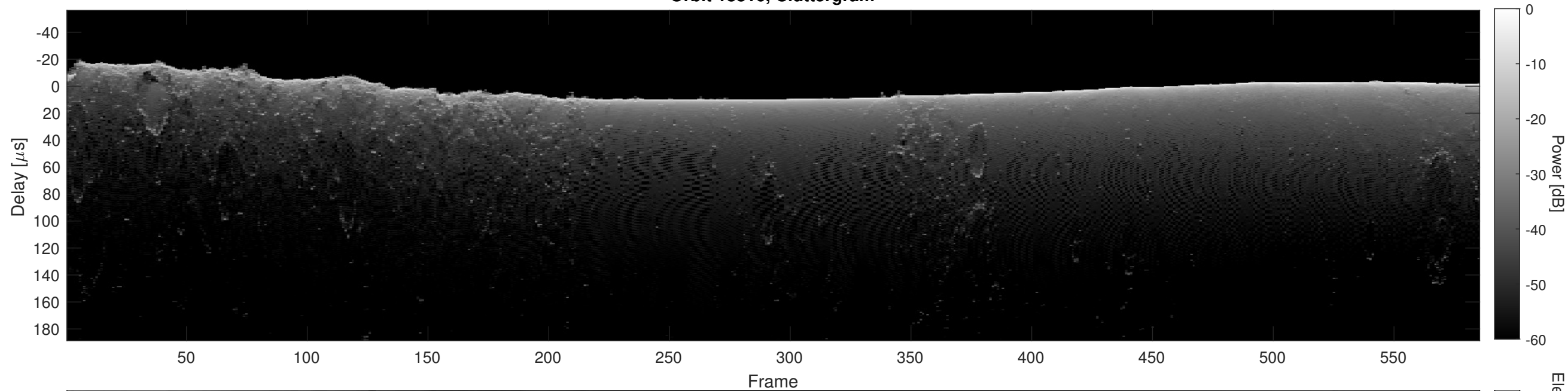
Orbit 18816, Cluttergram
