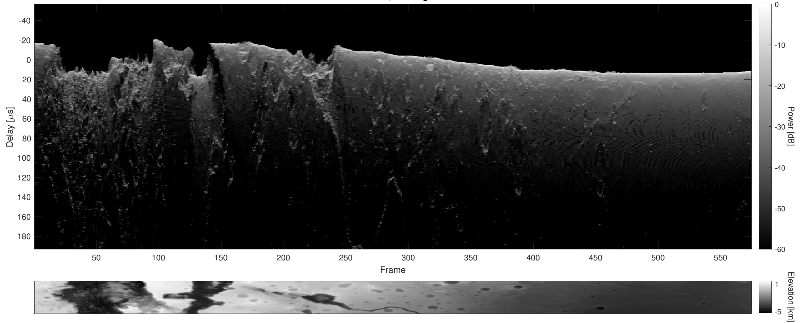
Orbit 18818, Cluttergram
