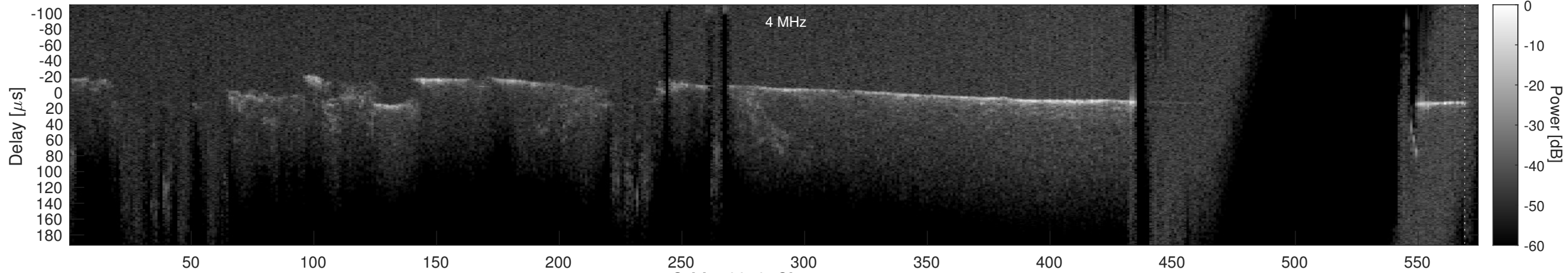
Orbit 18818, Cluttergram
