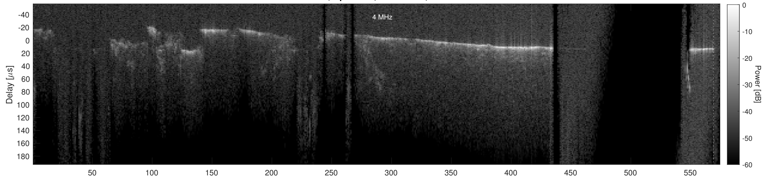
Orbit 18818, Cluttergram
