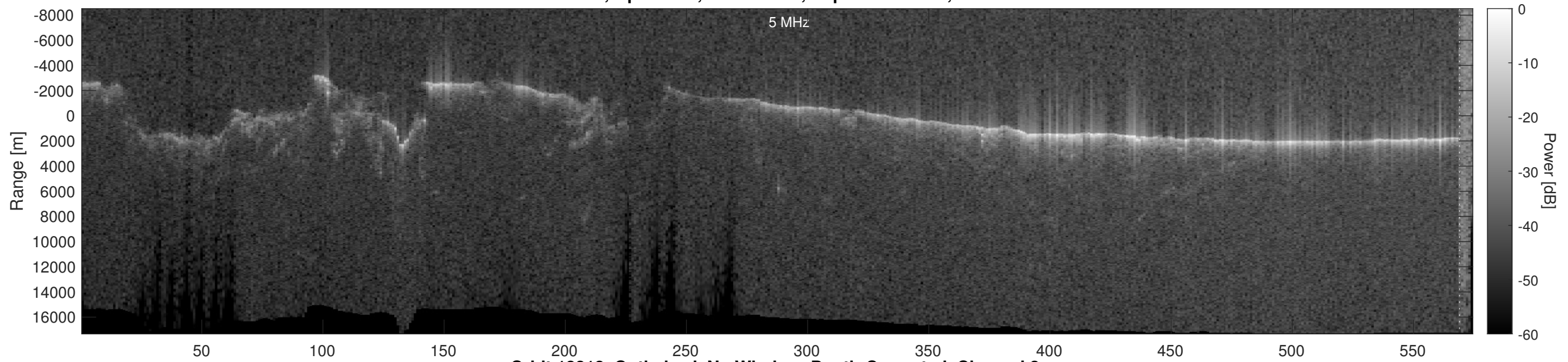
Orbit 18818, Optimized, No Window, Depth-Corrected, Channel 2
