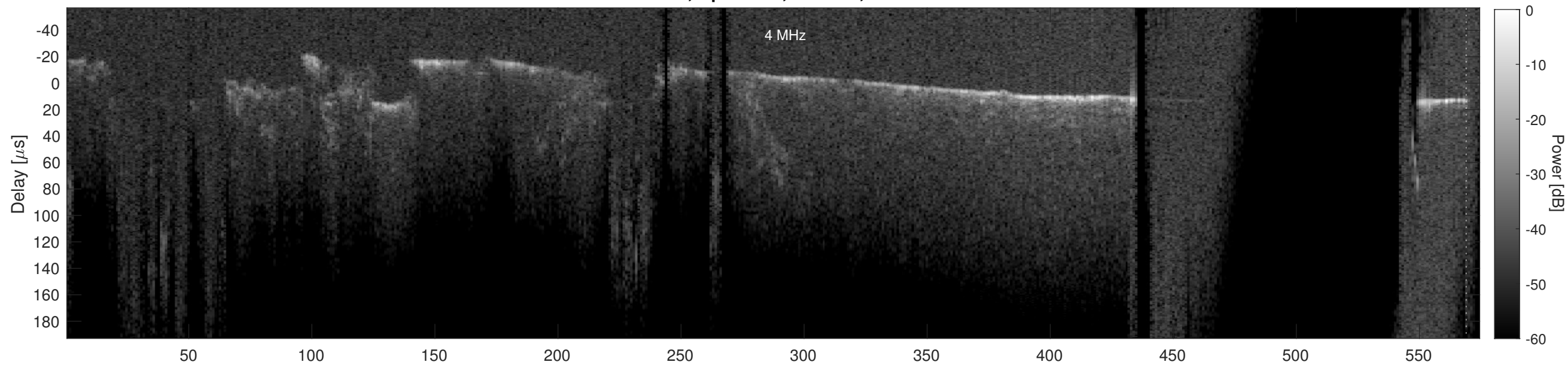
Orbit 18818, Cluttergram
