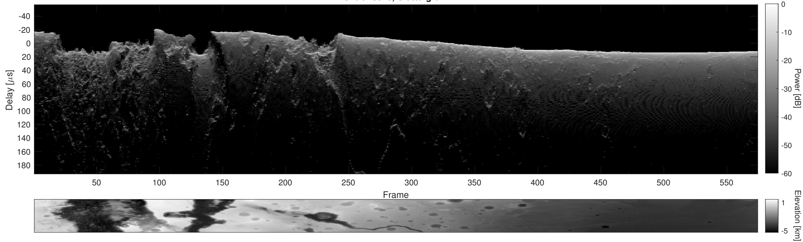
Orbit 18818, Cluttergram
