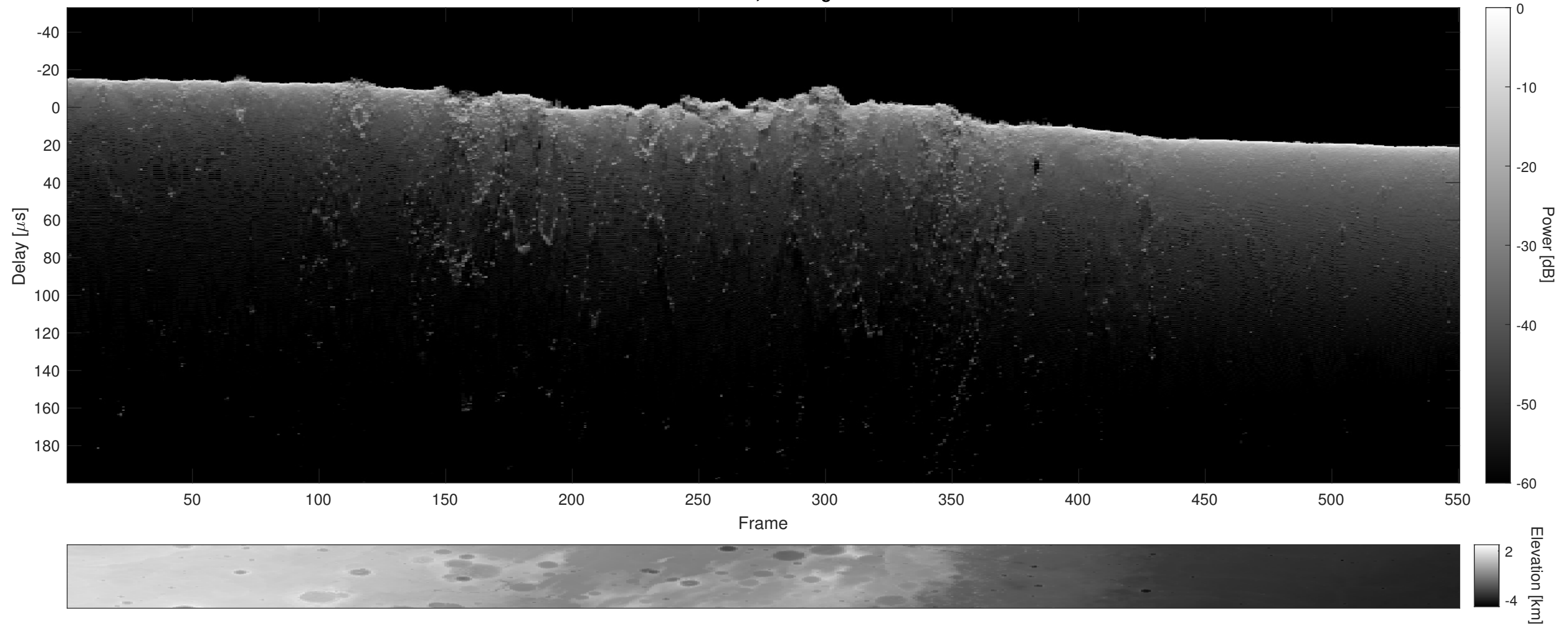
Orbit 18820, Cluttergram
