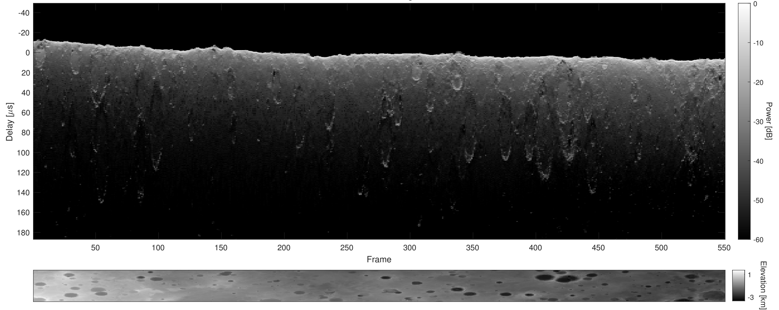
Orbit 18821, Cluttergram
