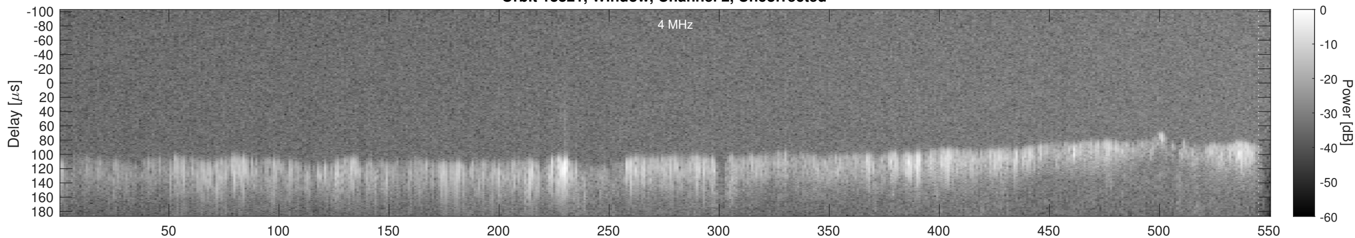
Orbit 18821, Window, Channel 2, Chapman
