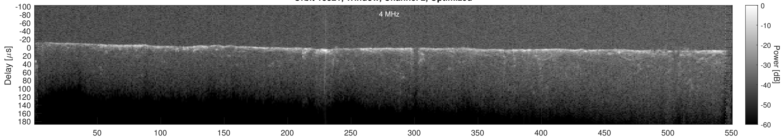
Orbit 18821, Cluttergram
