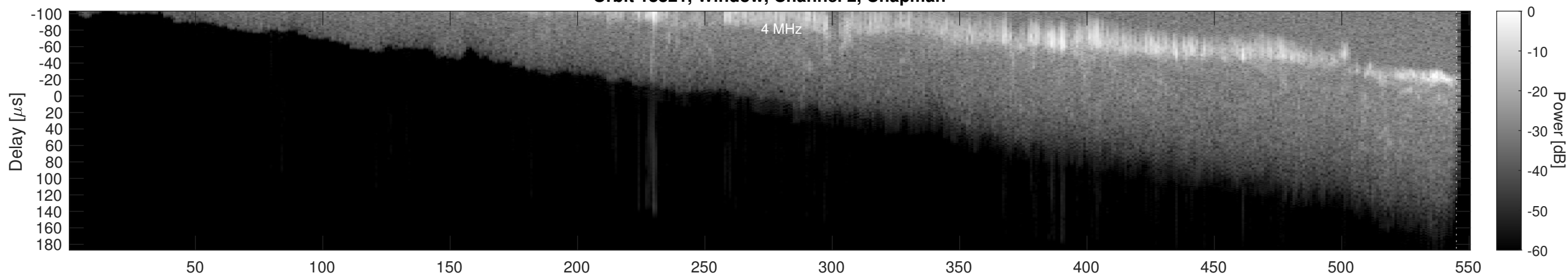
Orbit 18821, Window, Channel 2, Optimized
