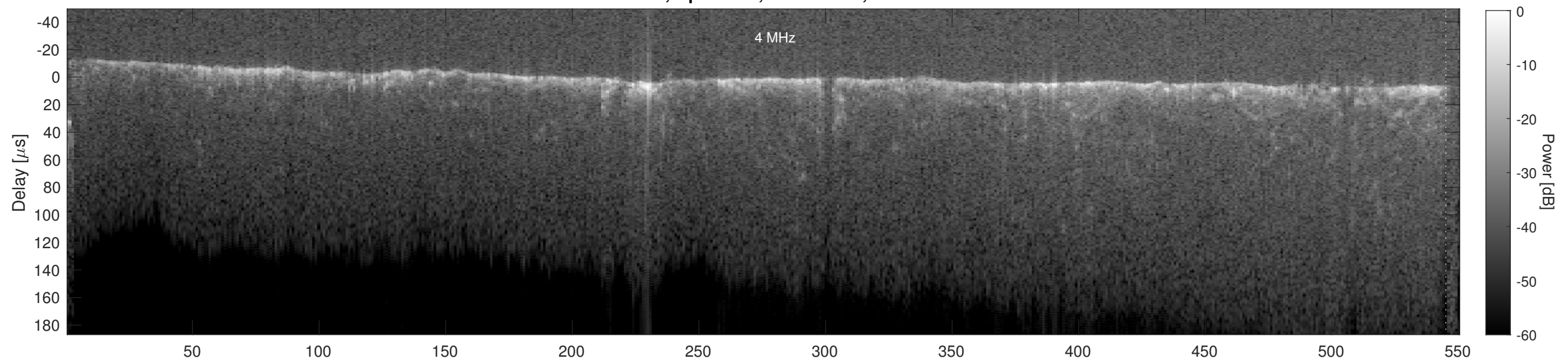
Orbit 18821, Cluttergram
