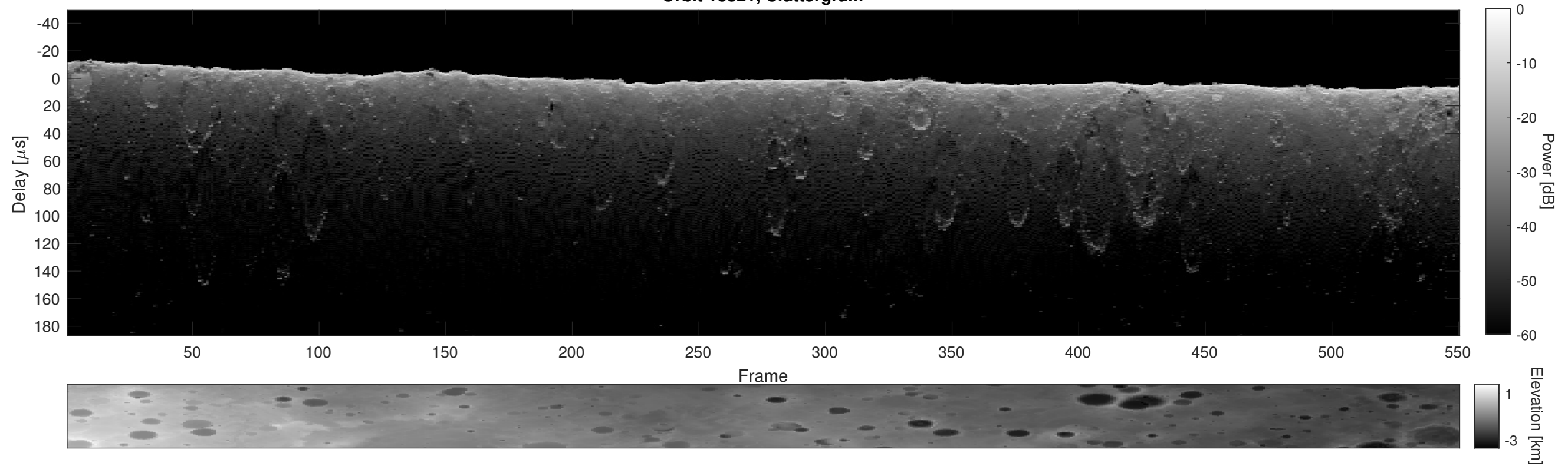
Orbit 18821, Cluttergram
