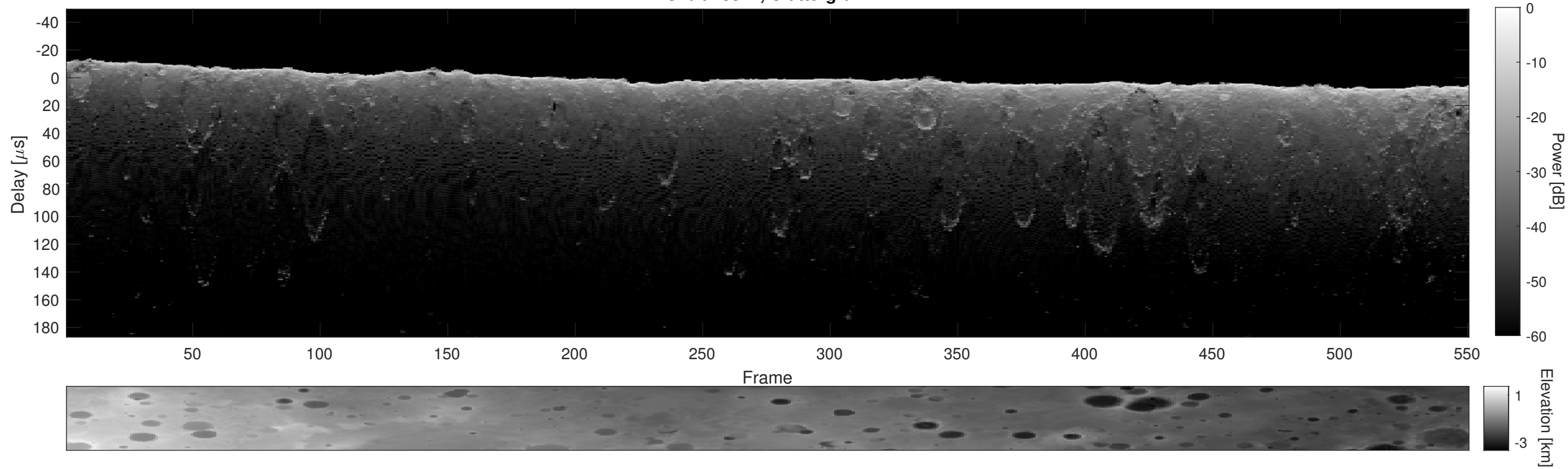
Orbit 18821, Cluttergram
