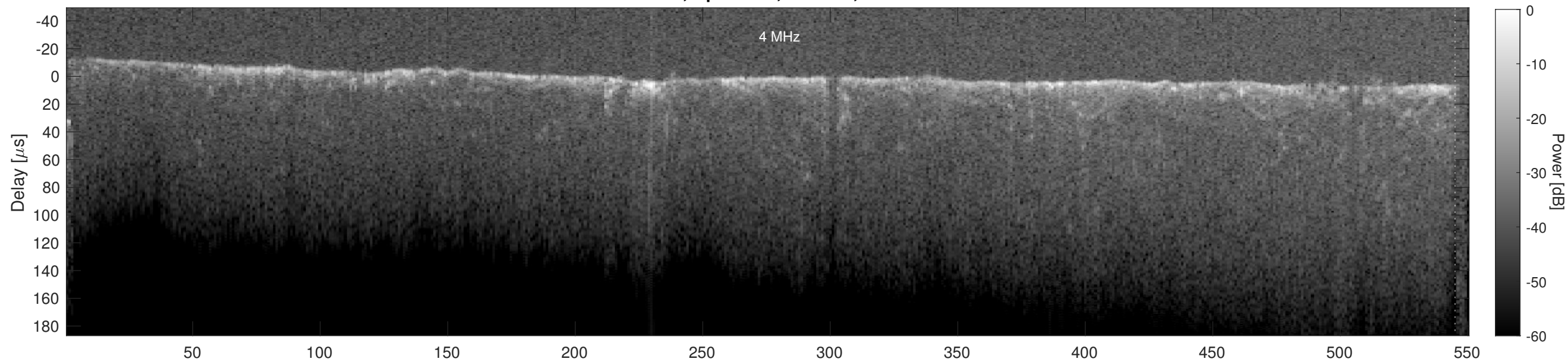
Orbit 18821, Cluttergram
