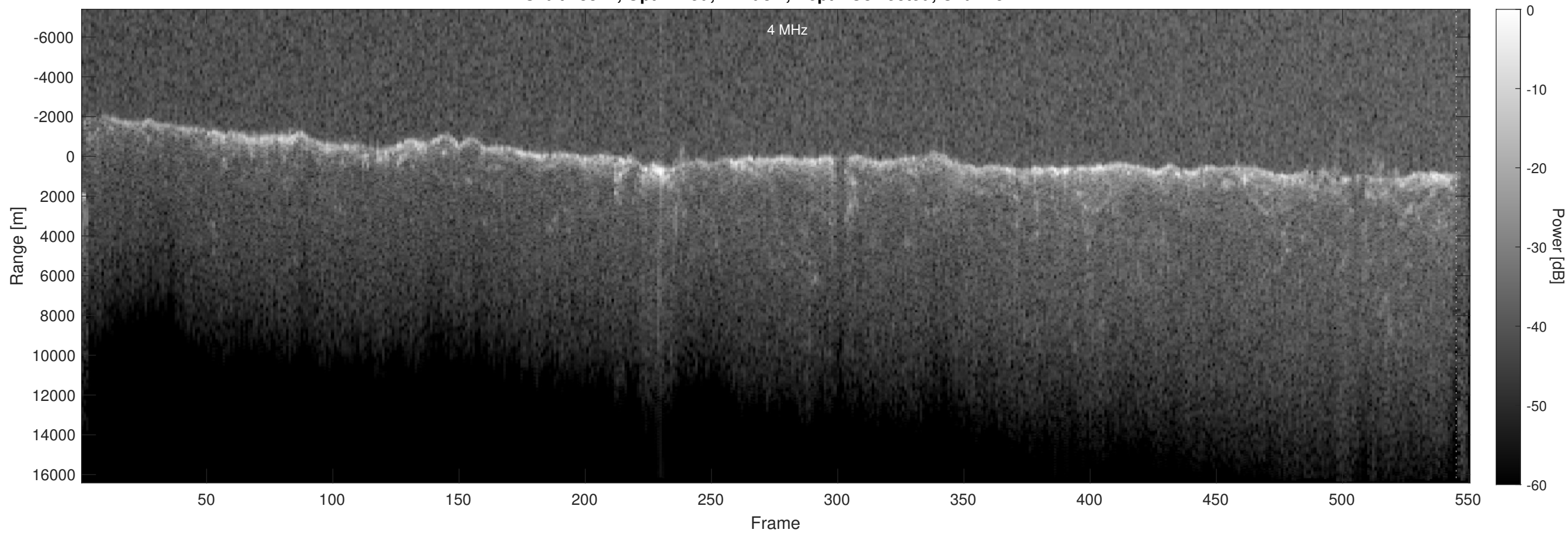
Orbit 18821, Optimized, Window, Depth-Corrected, Channel 2
