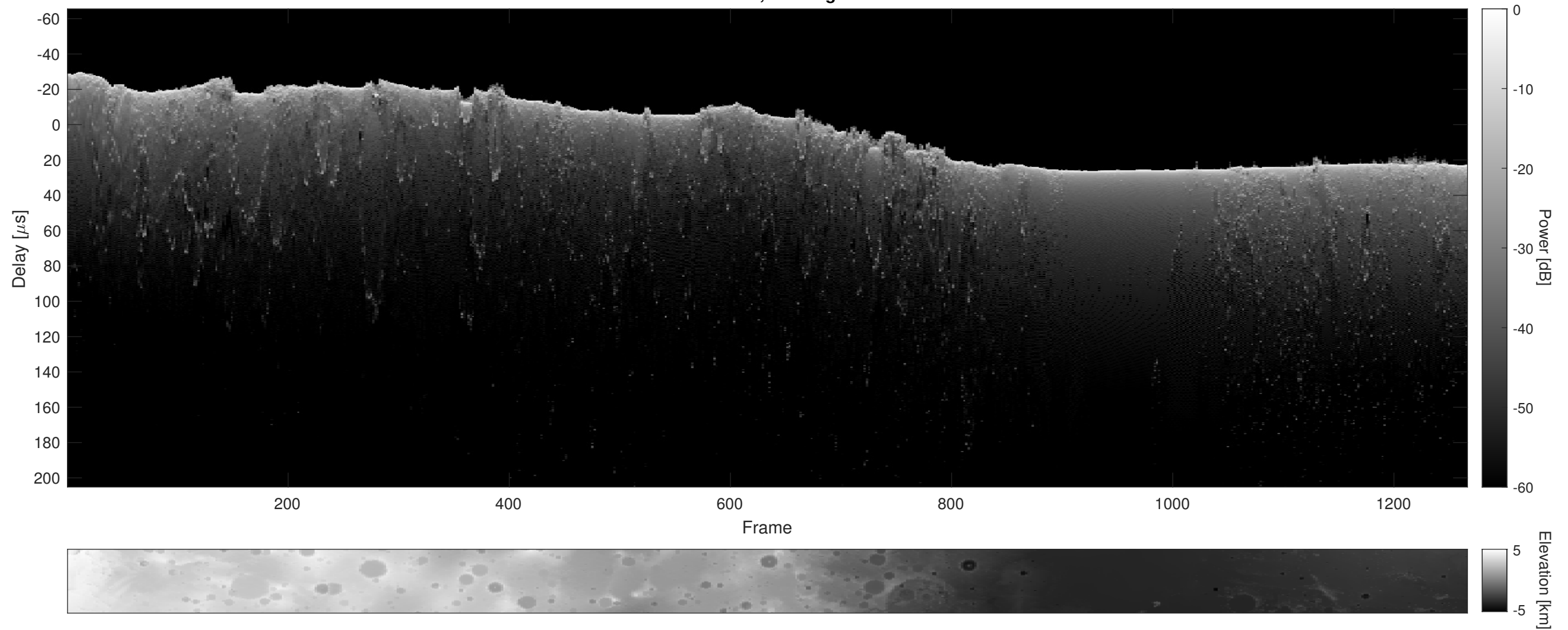
Orbit 18830, Cluttergram
