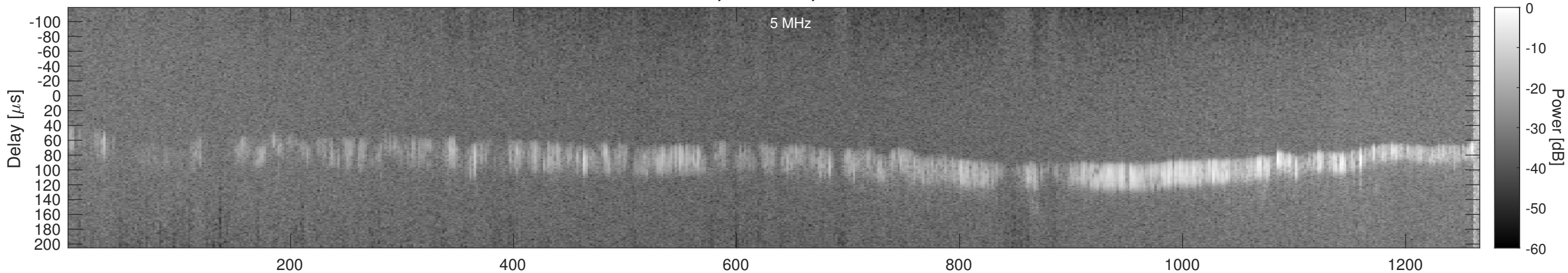
Orbit 18830, Window, Channel 1, Chapman
