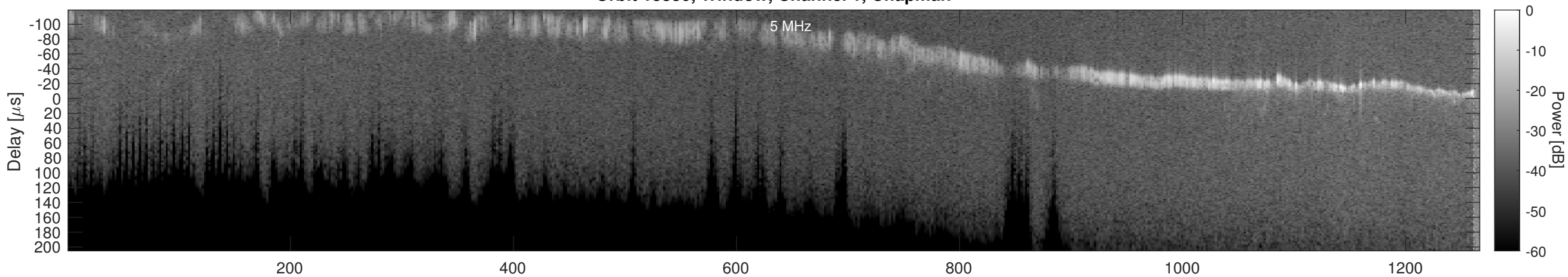
Orbit 18830, Window, Channel 1, Optimized
