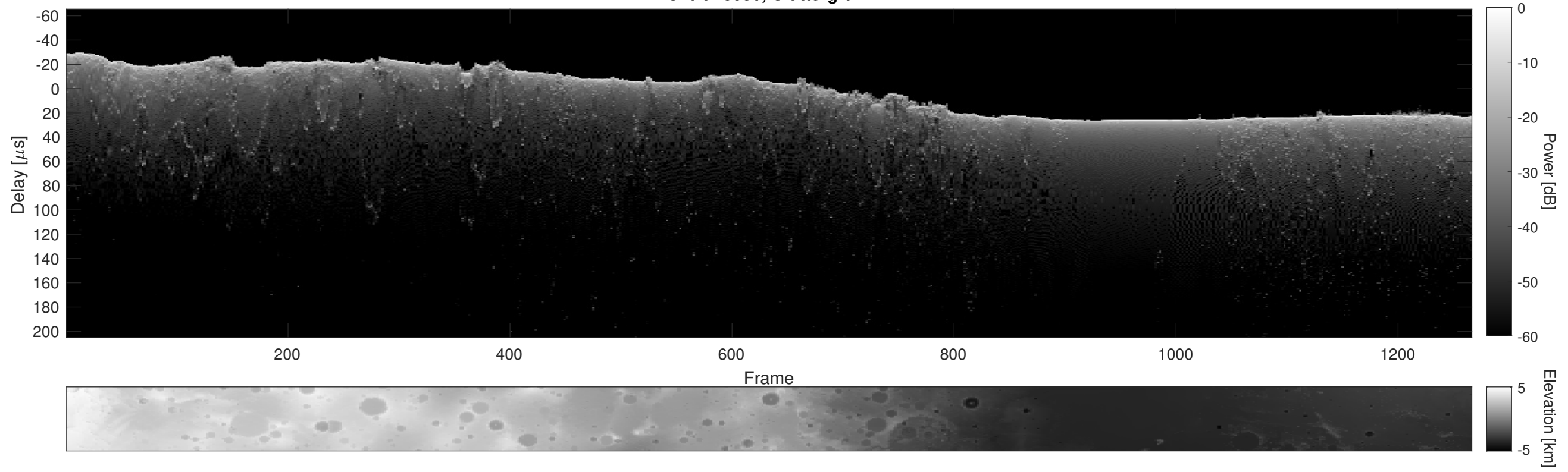
Orbit 18830, Cluttergram
