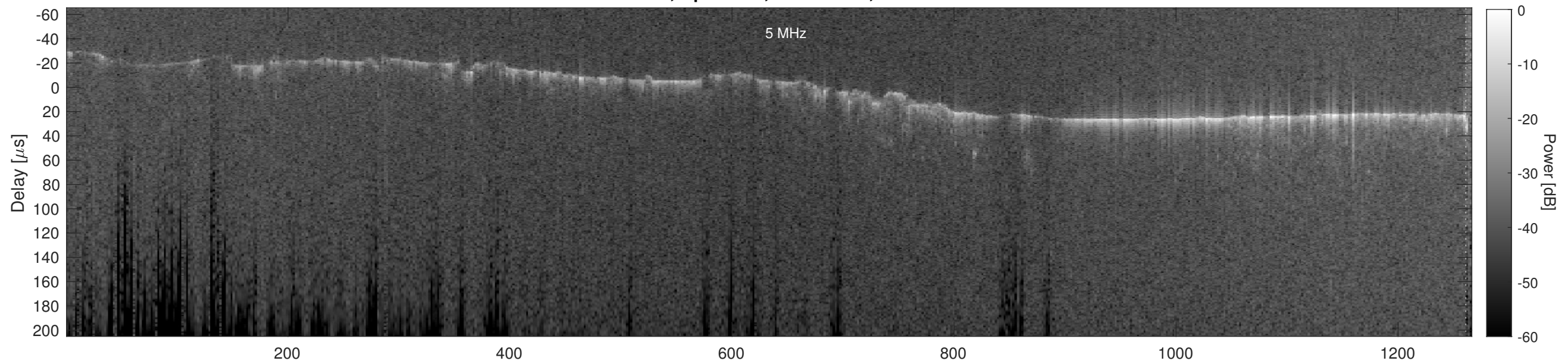
Orbit 18830, Cluttergram
