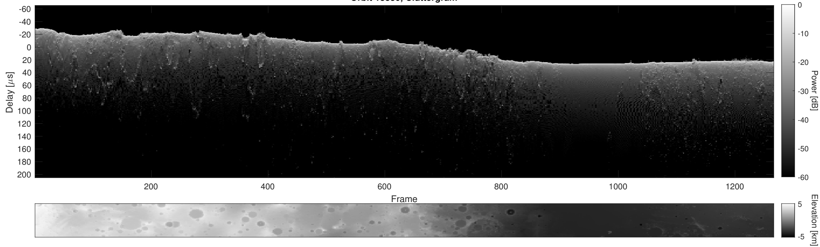
Orbit 18830, Cluttergram
