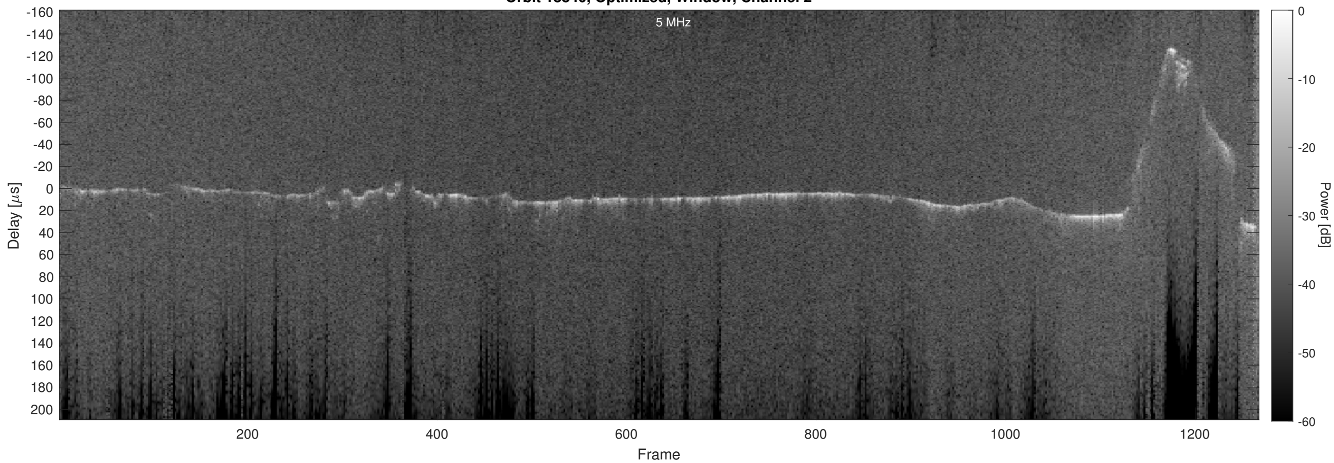
Orbit 18840, Optimized, Window, Channel 2
