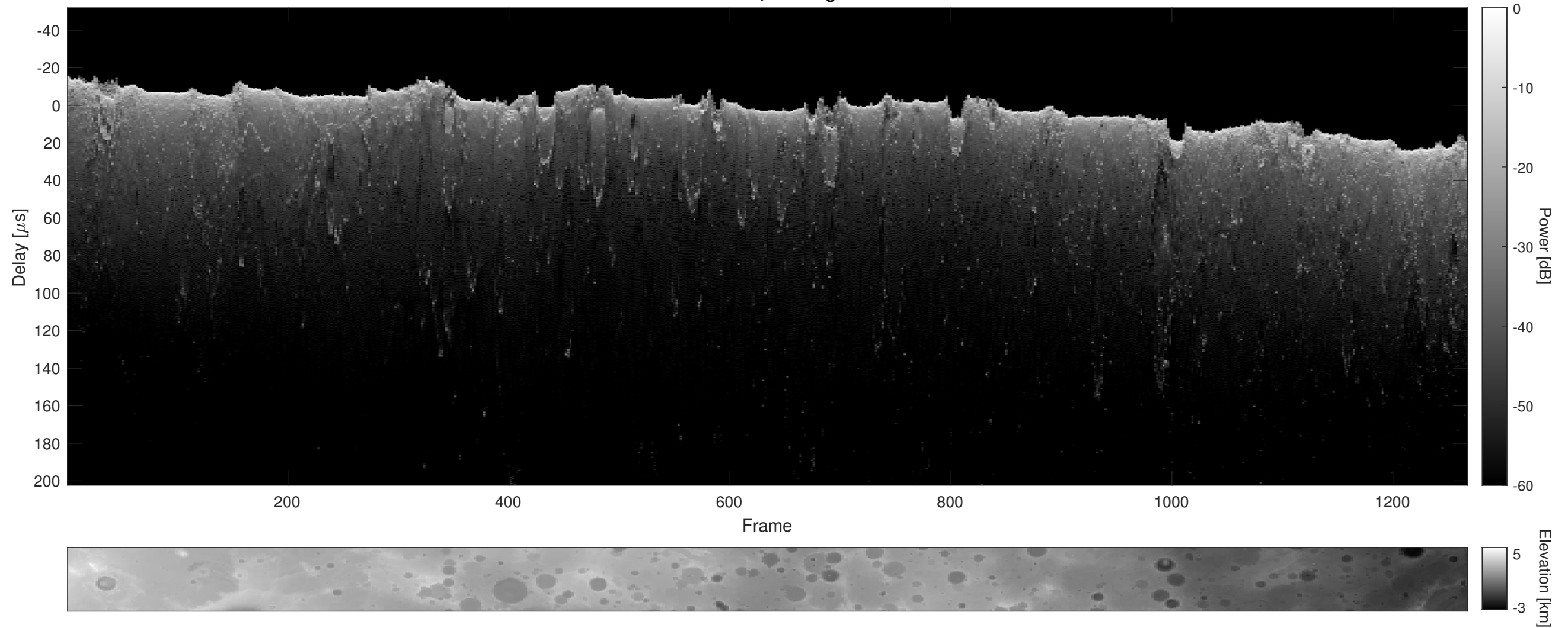
Orbit 18849, Cluttergram
