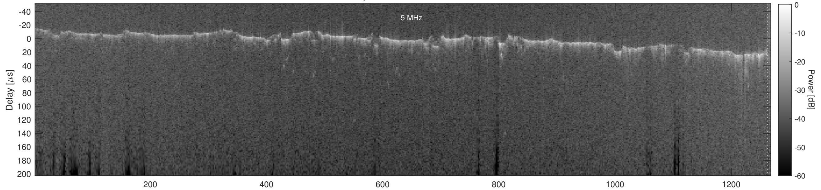
Orbit 18849, Cluttergram
