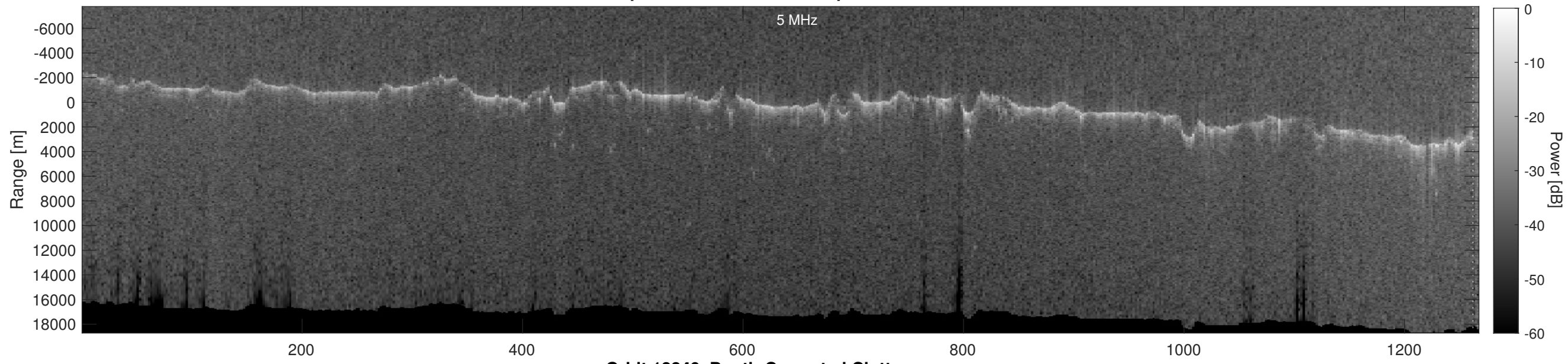
Orbit 18849, Depth-Corrected Cluttergram
