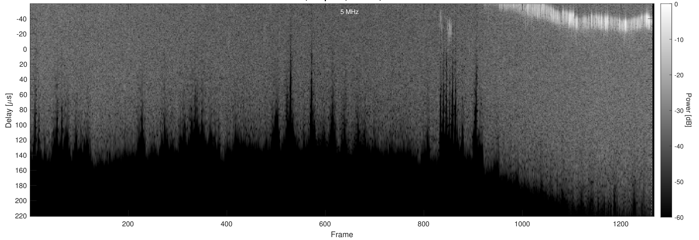
Orbit 18864, Chapman, Window, Channel 2
