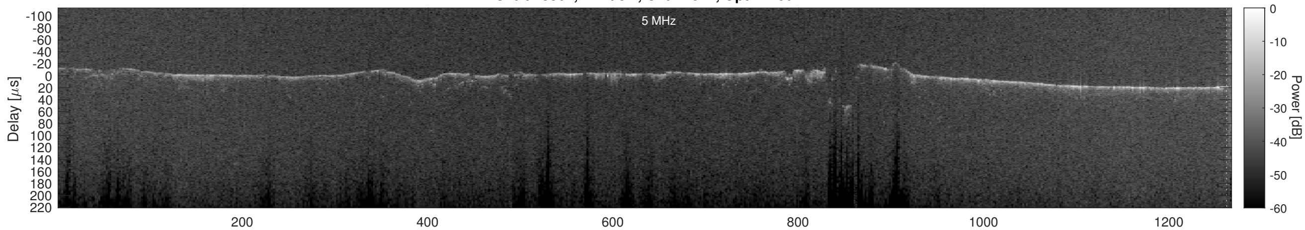
Orbit 18864, Cluttergram
