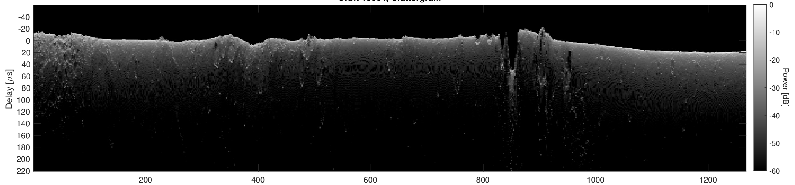
Orbit 18864, Cluttergram
