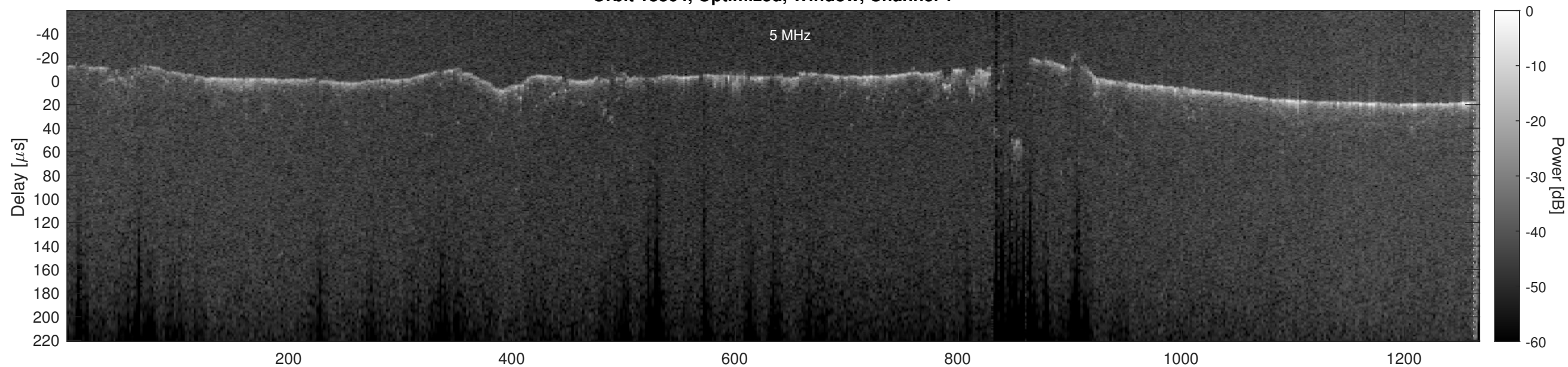
Orbit 18864, Optimized, Window, Channel 2
