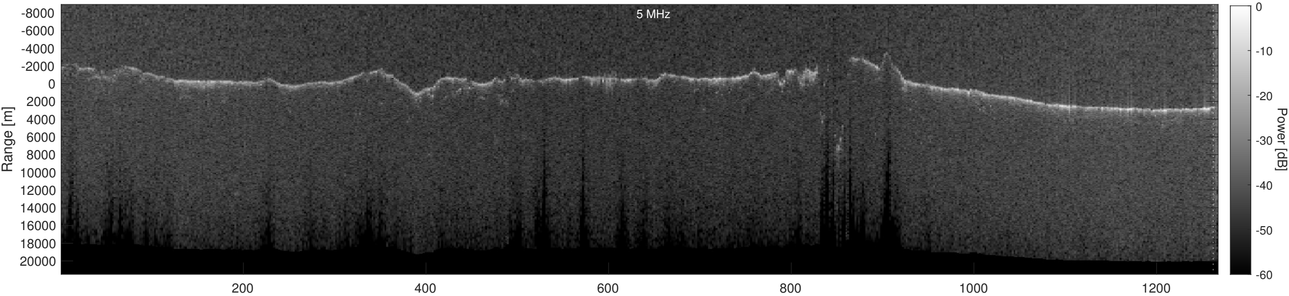
Orbit 18864, Depth-Corrected Cluttergram
