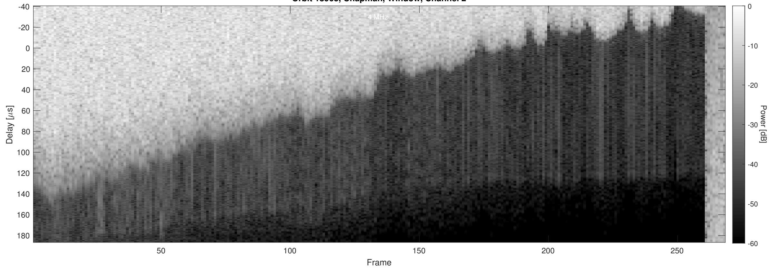
Orbit 18963, Chapman, Window, Channel 2
