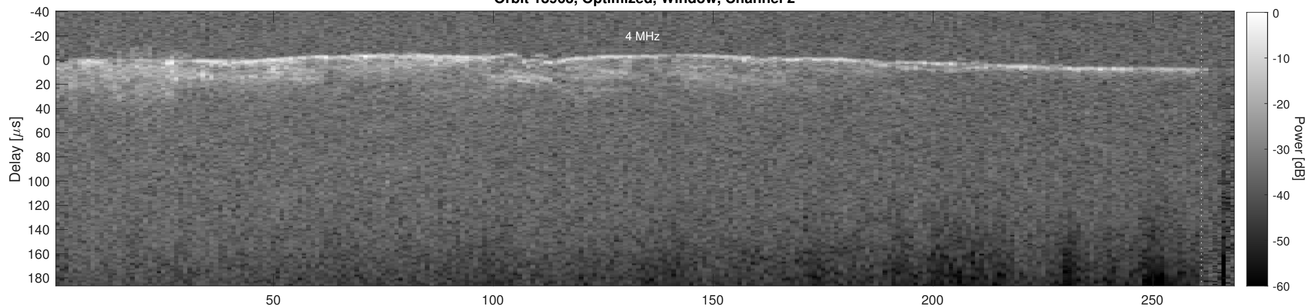
Orbit 18963, Cluttergram
