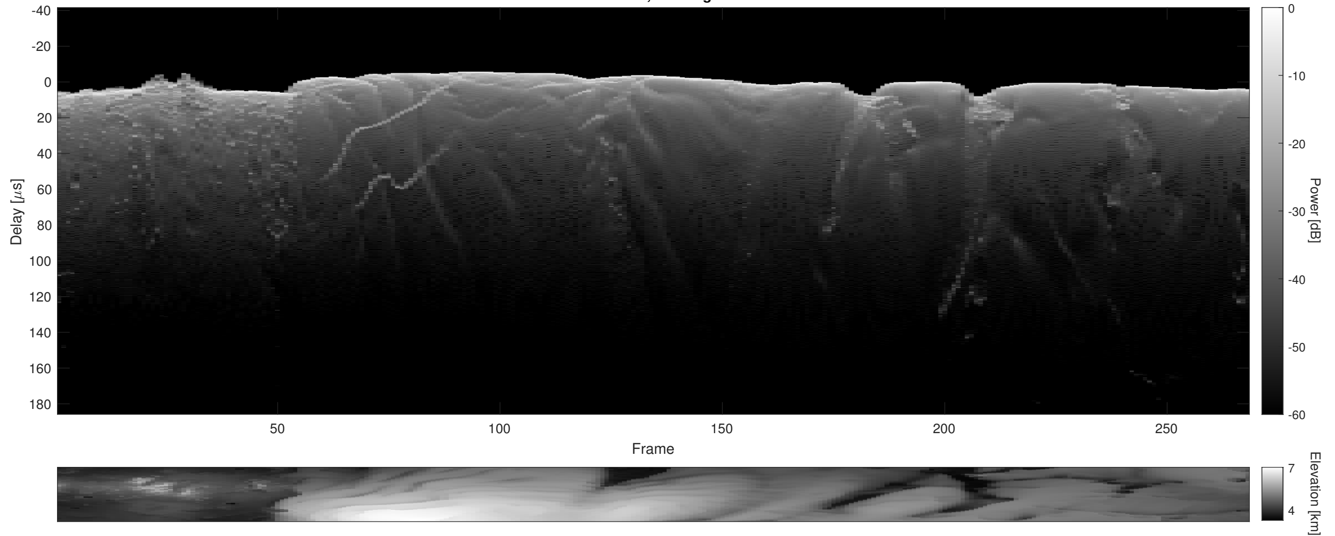
Orbit 18964, Cluttergram
