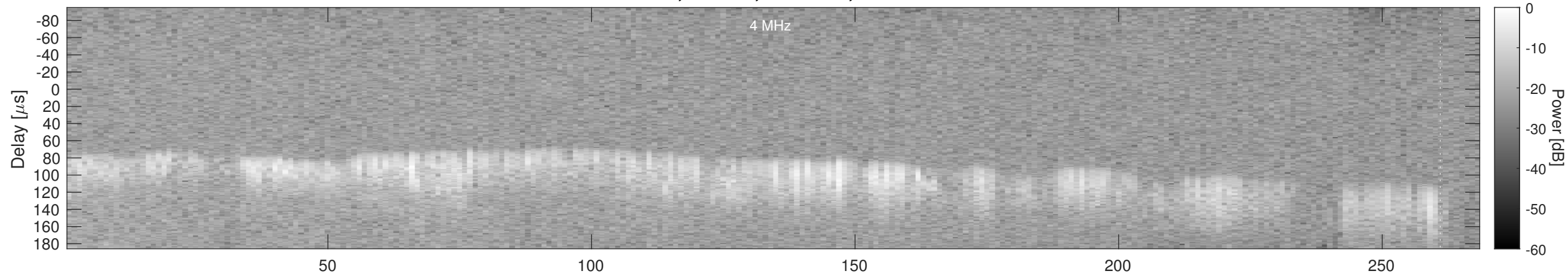
Orbit 18964, Window, Channel 2, Chapman
