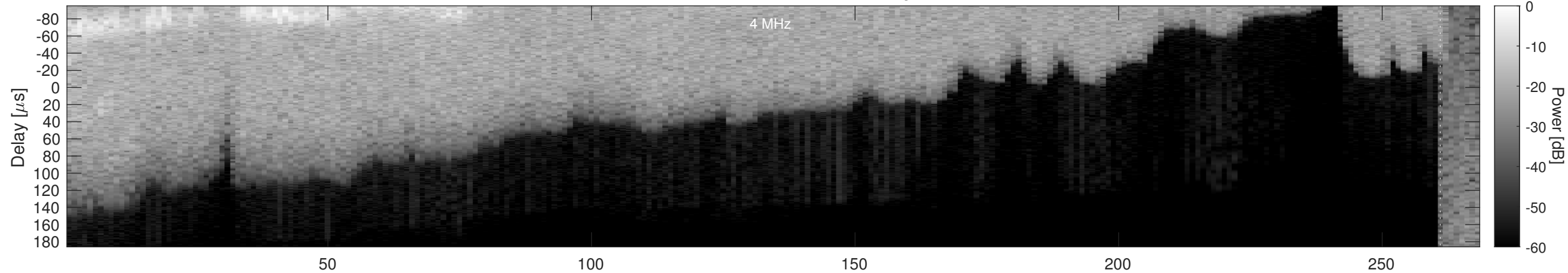
Orbit 18964, Window, Channel 2, Optimized
