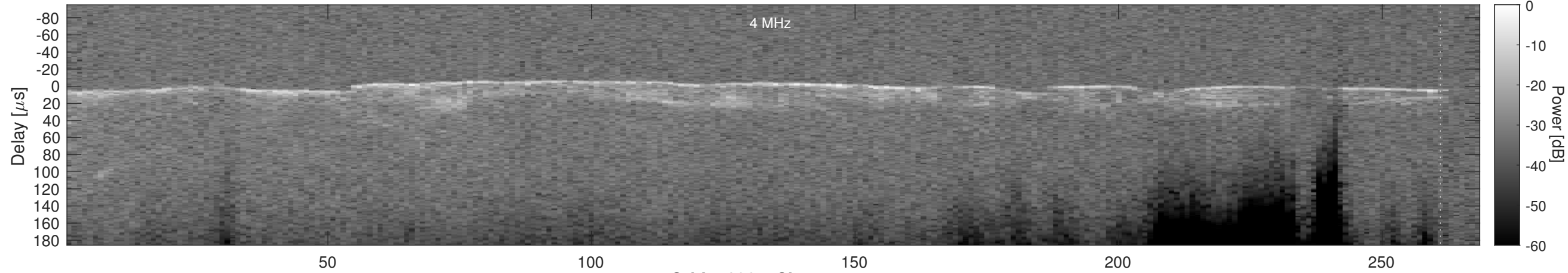
Orbit 18964, Cluttergram
