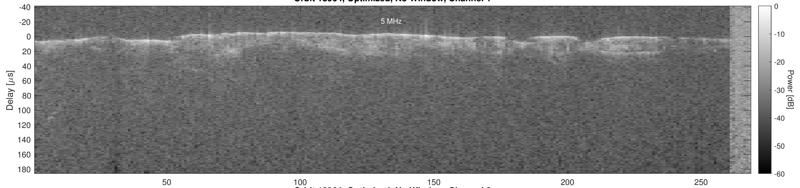
Orbit 18964, Optimized, No Window, Channel 2
