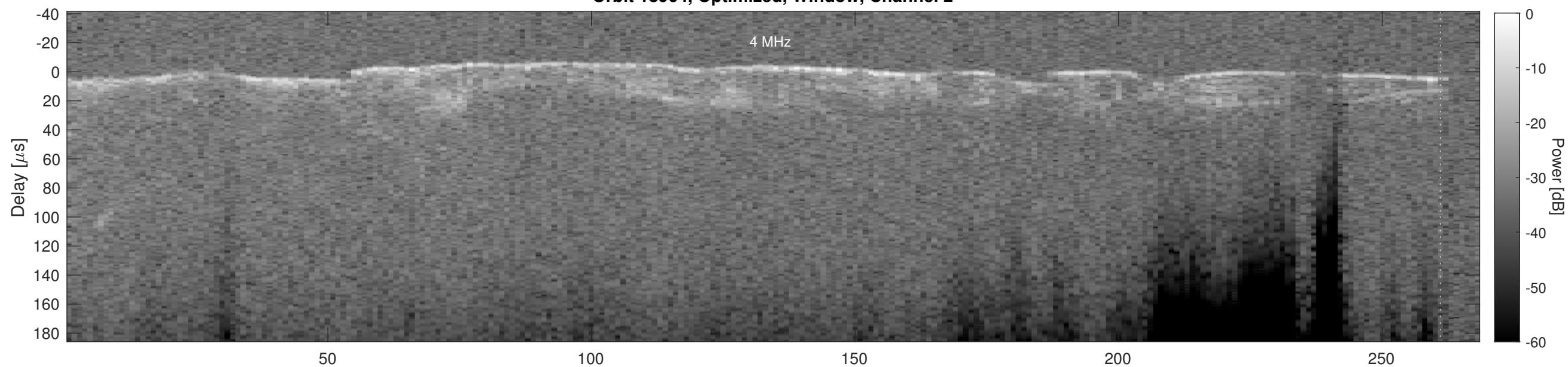
Orbit 18964, Cluttergram
