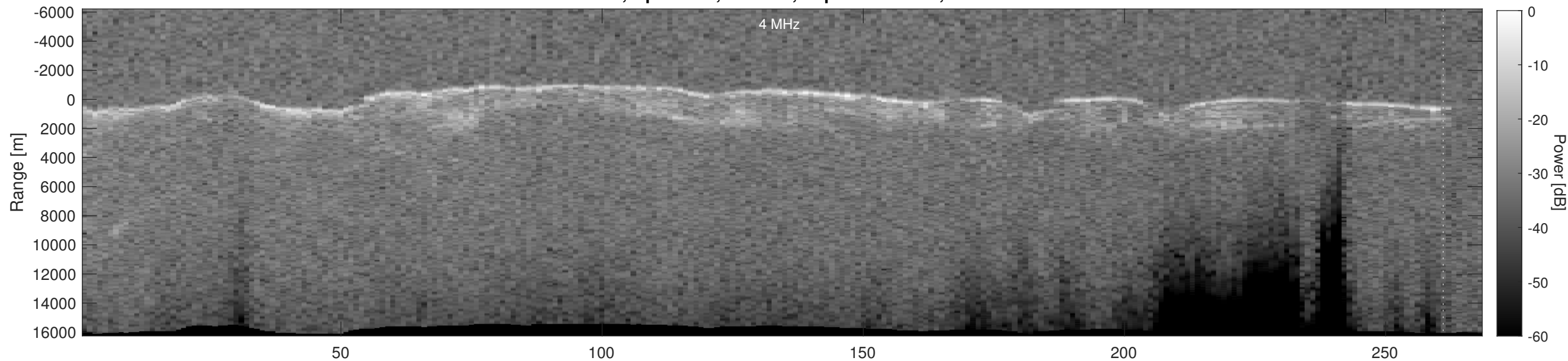
Orbit 18964, Depth-Corrected Cluttergram
