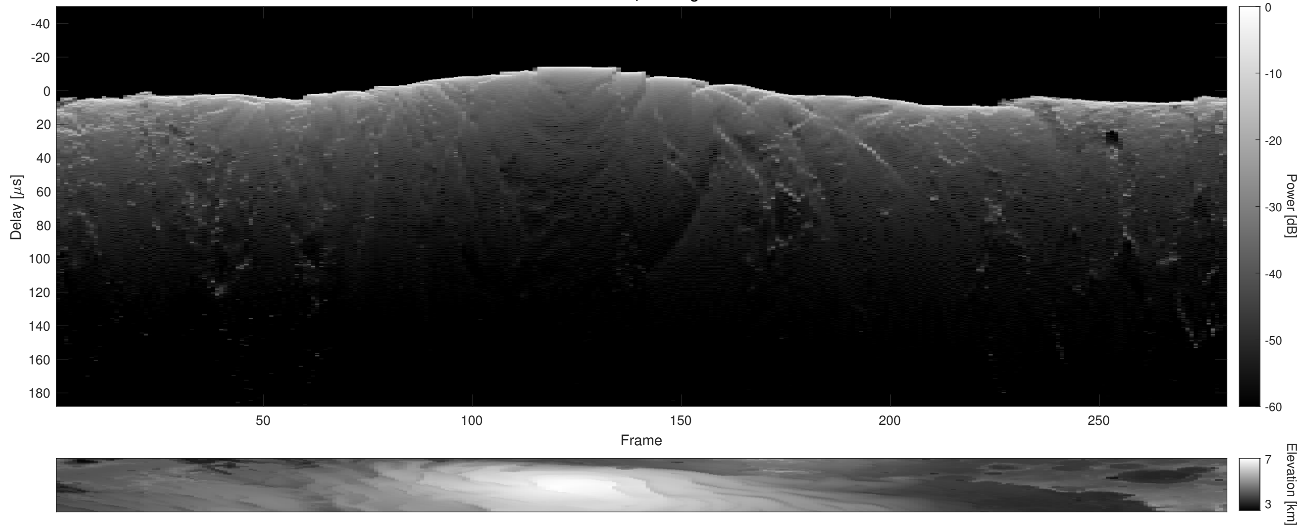
Orbit 18965, Cluttergram
