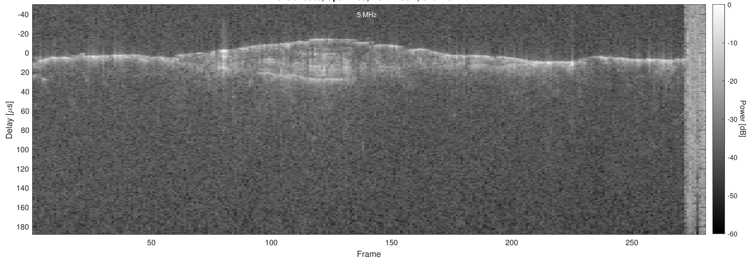
Orbit 18965, Optimized, No Window, Channel 2
