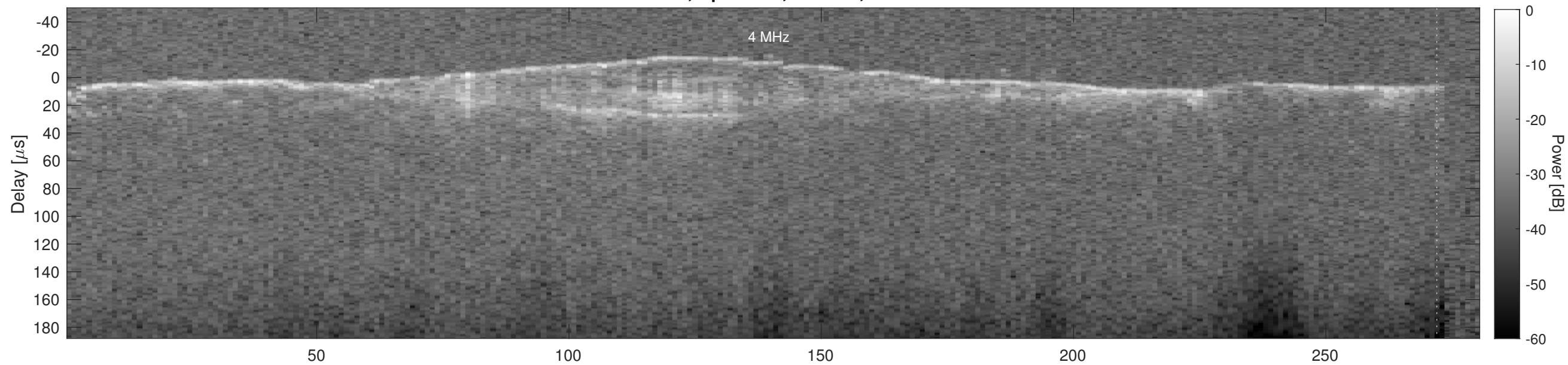
Orbit 18965, Cluttergram
