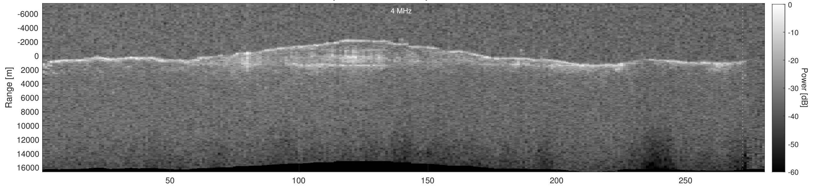
Orbit 18965, Depth-Corrected Cluttergram
