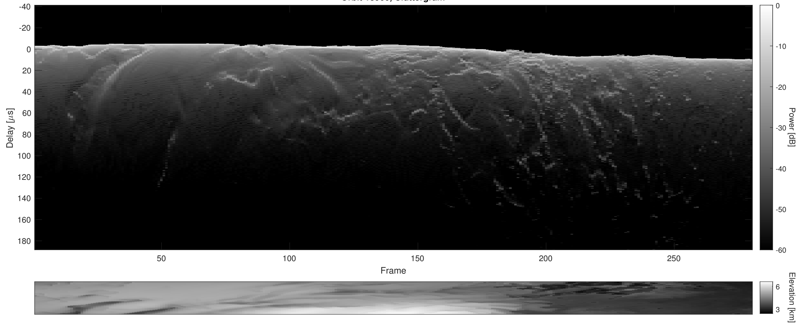
Orbit 18966, Cluttergram
