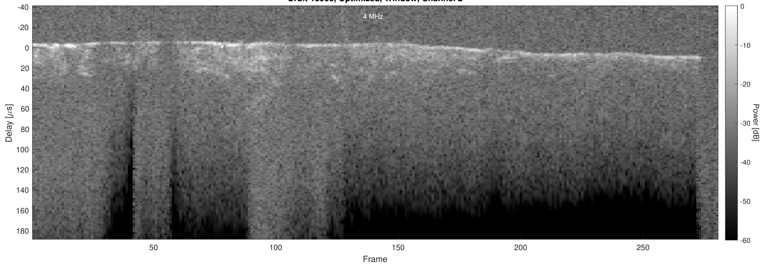
Orbit 18966, Optimized, Window, Channel 2
