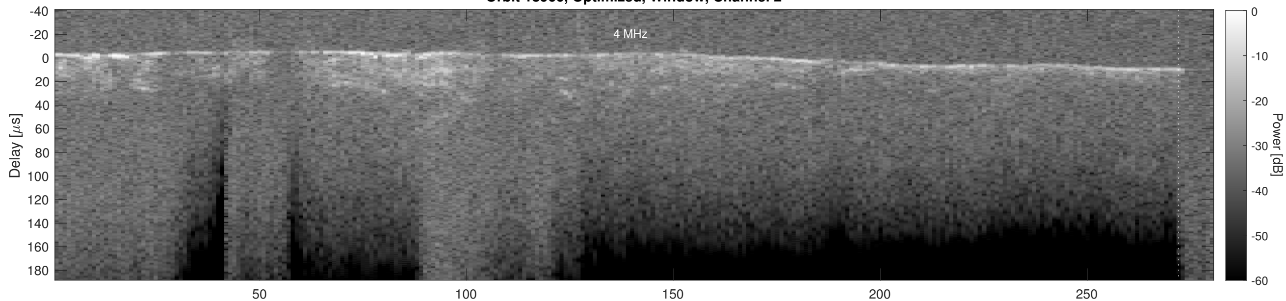
Orbit 18966, Cluttergram
