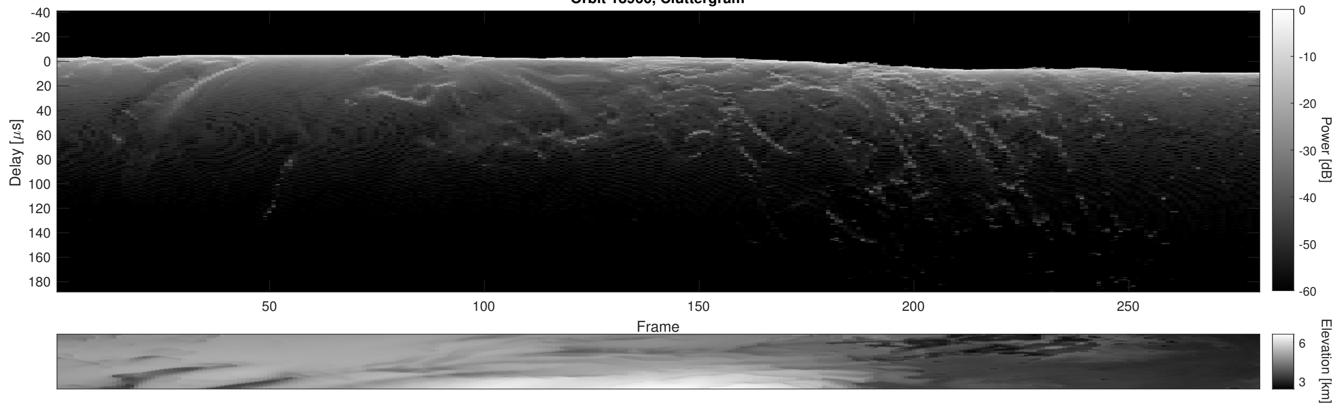
Orbit 18966, Cluttergram
