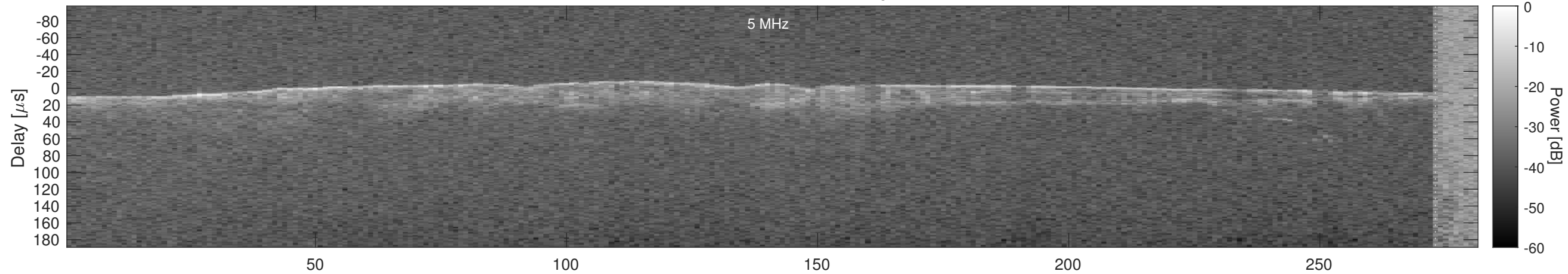
Orbit 18967, Cluttergram
