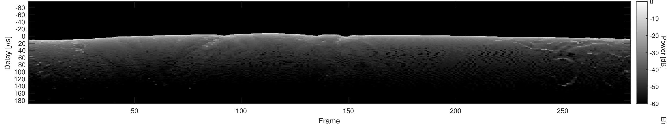
Orbit 18967, Cluttergram
