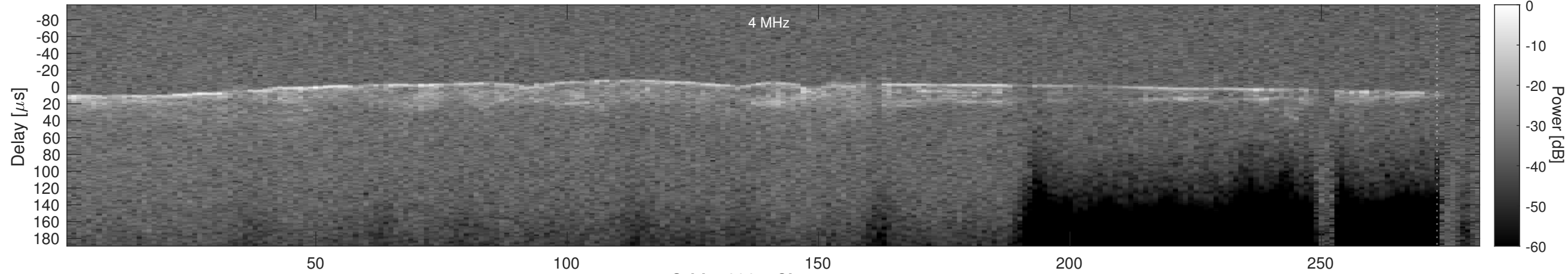
Orbit 18967, Cluttergram
