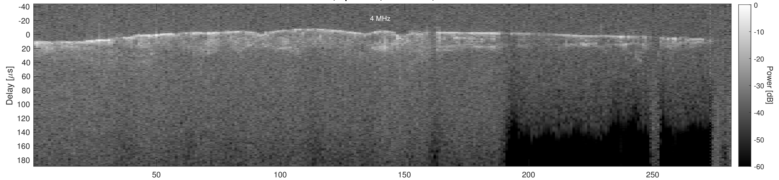
Orbit 18967, Cluttergram
