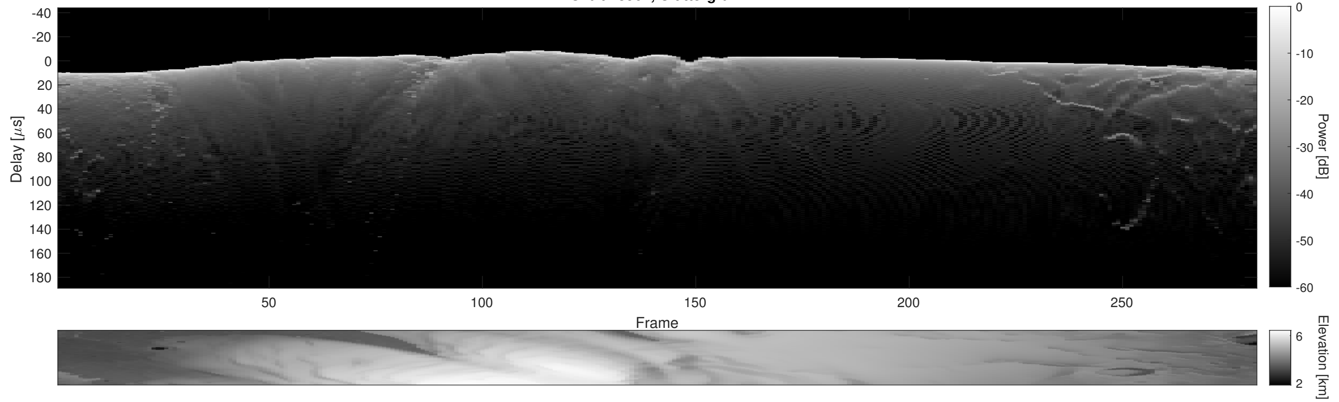
Orbit 18967, Cluttergram
