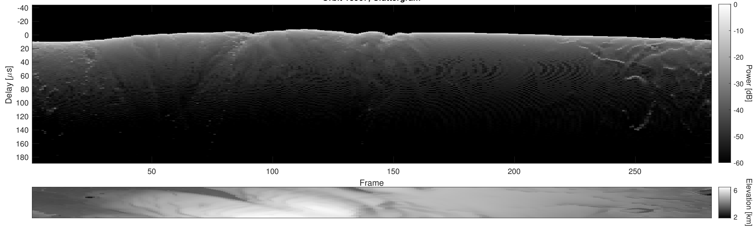
Orbit 18967, Cluttergram
