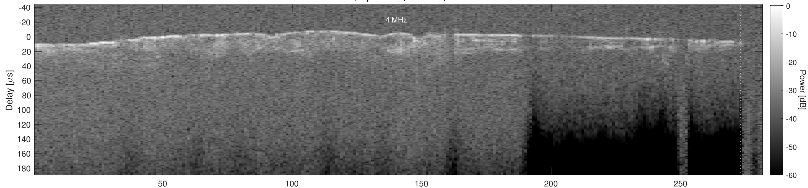
Orbit 18967, Cluttergram
