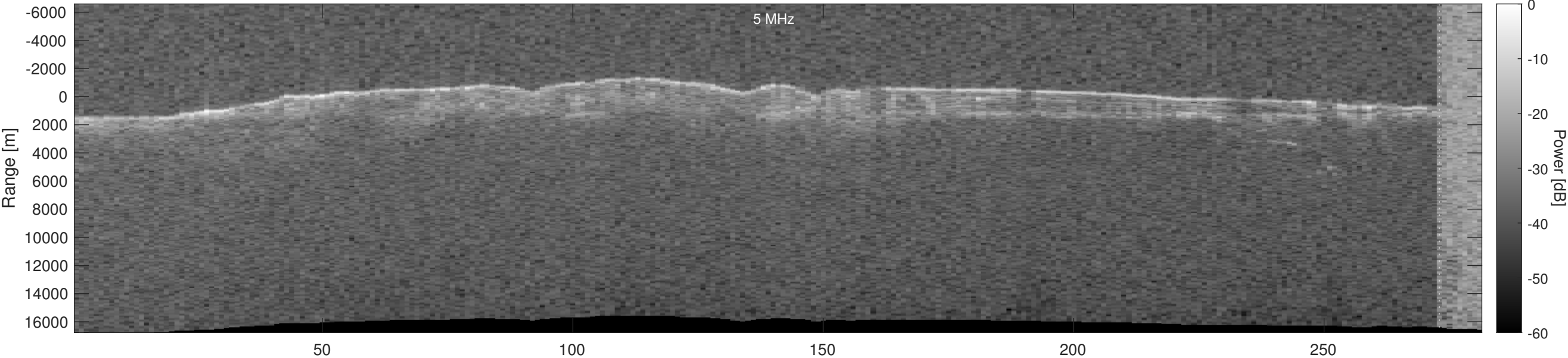
Orbit 18967, Optimized, Window, Depth-Corrected, Channel 2
