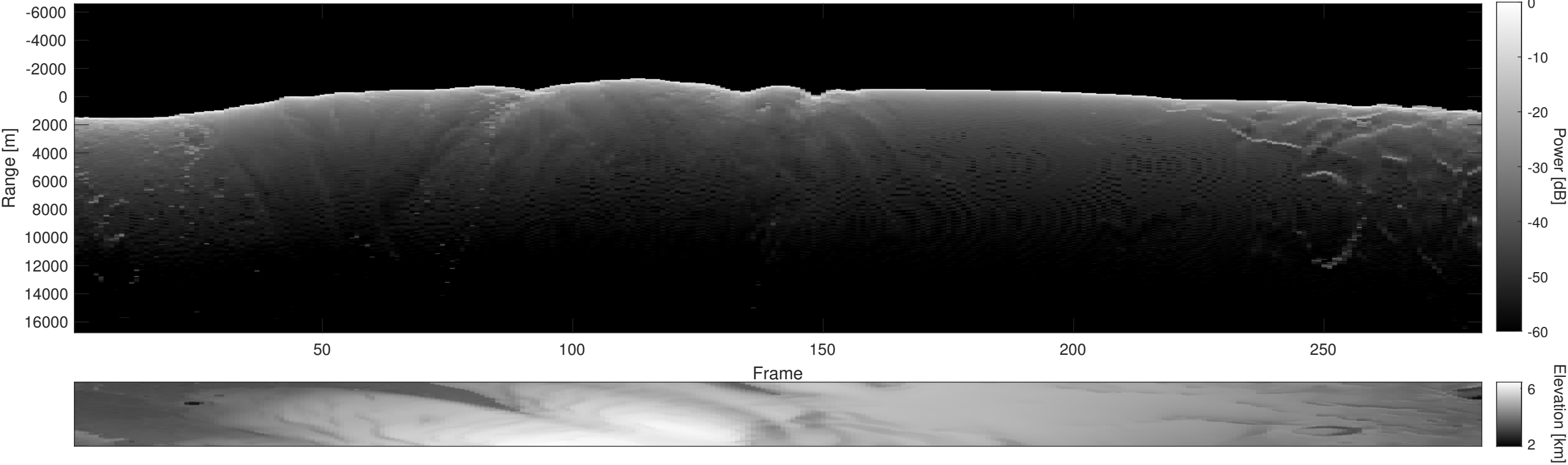
Orbit 18967, Depth-Corrected Cluttergram
