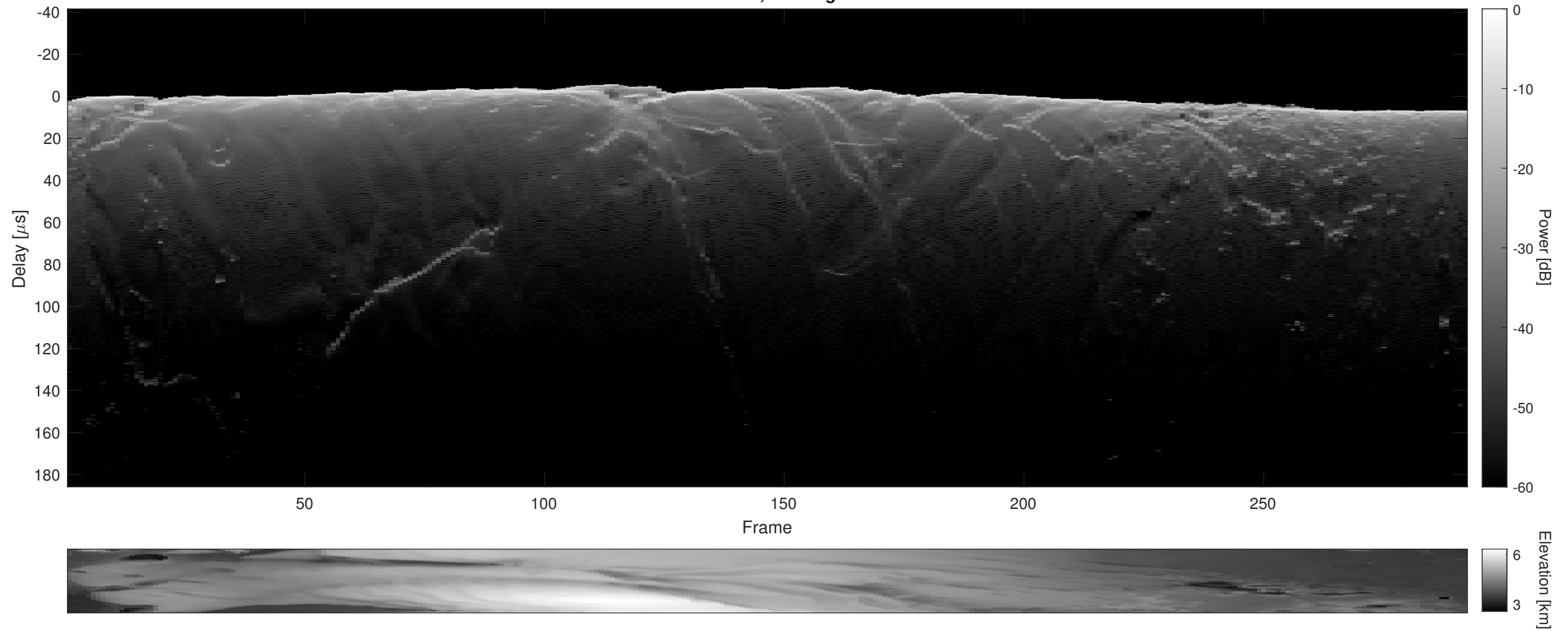
Orbit 18970, Cluttergram
